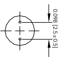
MOUNTING HOLES PATTERN
