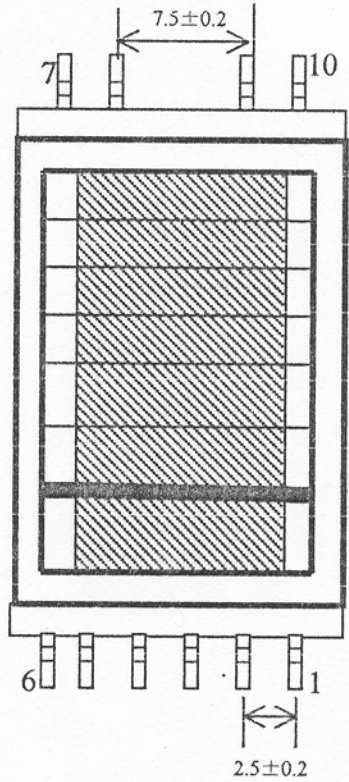
TOP VIEW
