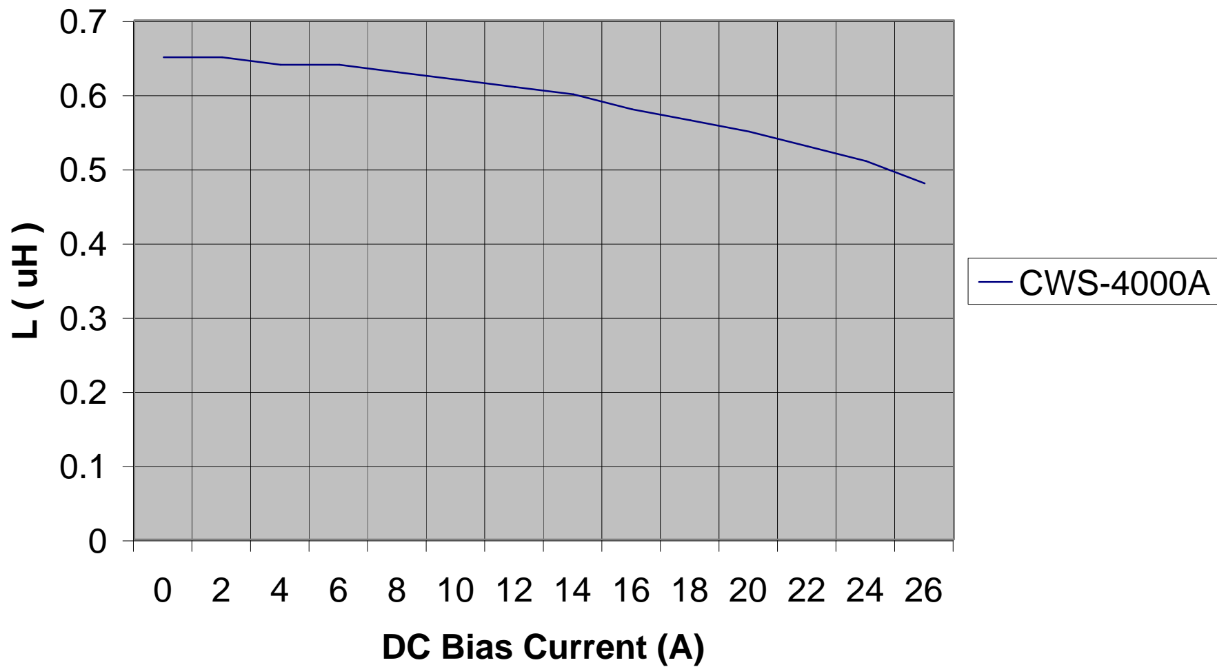
Inductance Versus DC Bias Current. 125 deg C
