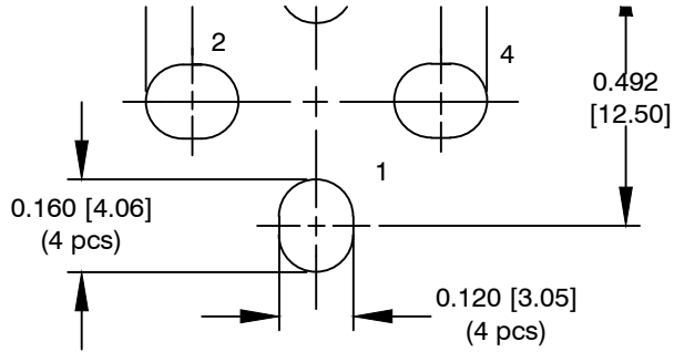
MOUNTING HOLES PATTERN
