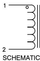
SCHEMATIC
